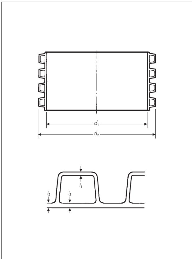
Figure 1 Ridgidrain pipe
