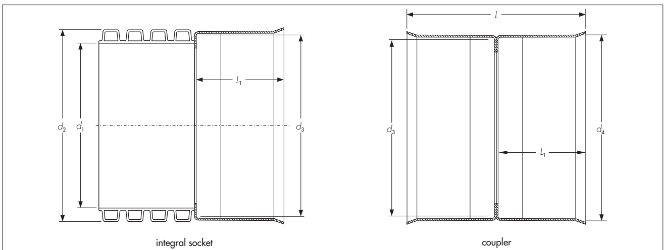
Figure 2 Welded integral socket and couplers
