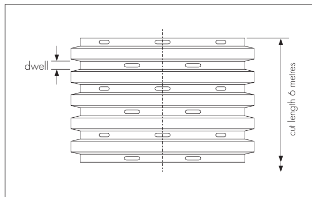
Figure 4 Details of perforations
